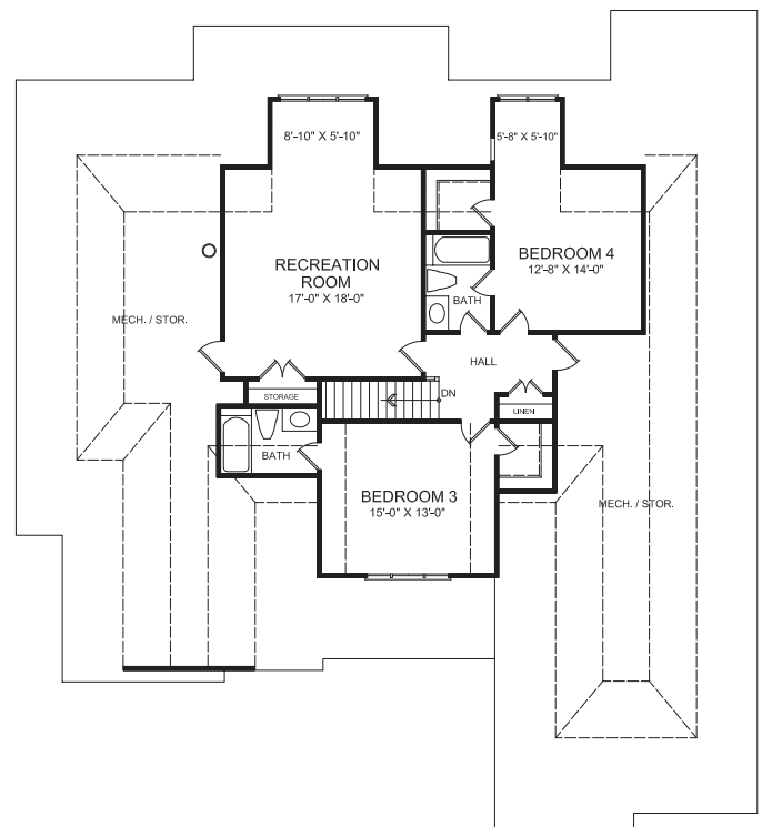
SECOND FLOOR
